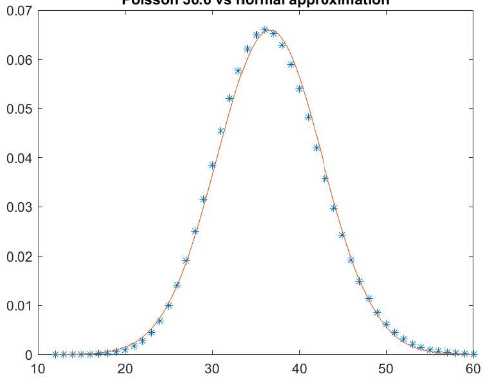
Poisson 36.6 vs normal approximation
