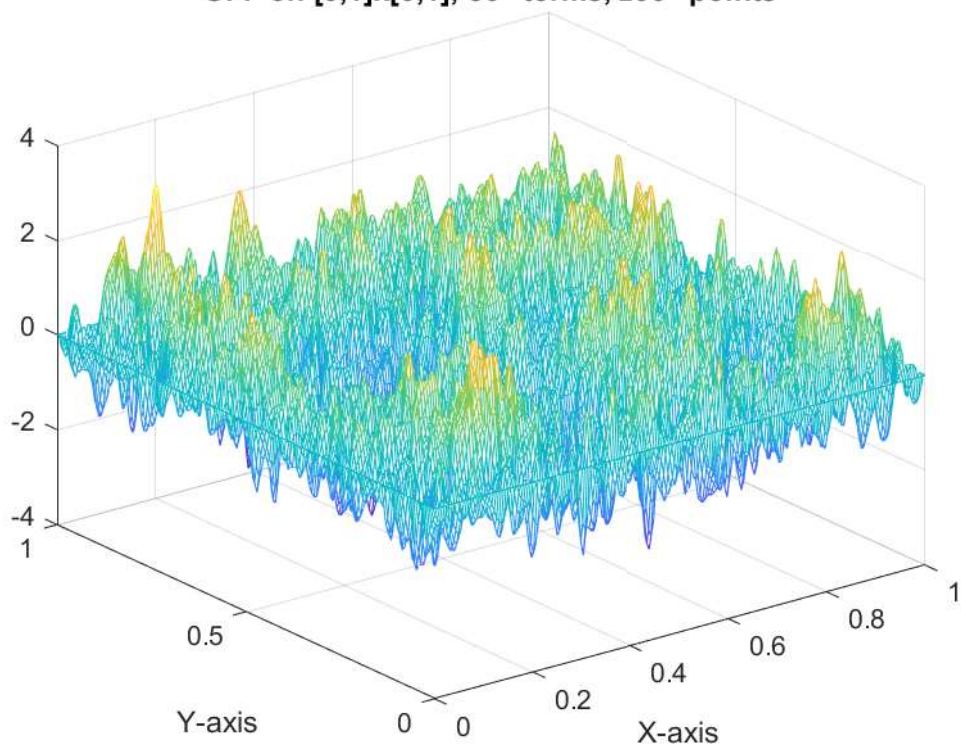
GFF on [0,1] \times [0,1] ; 80^2 terms, 200^2 points
