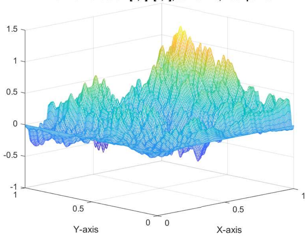
Brownian Sheet on [0,1] \times [0,1] ; 80^2 terms, 200^2 points
