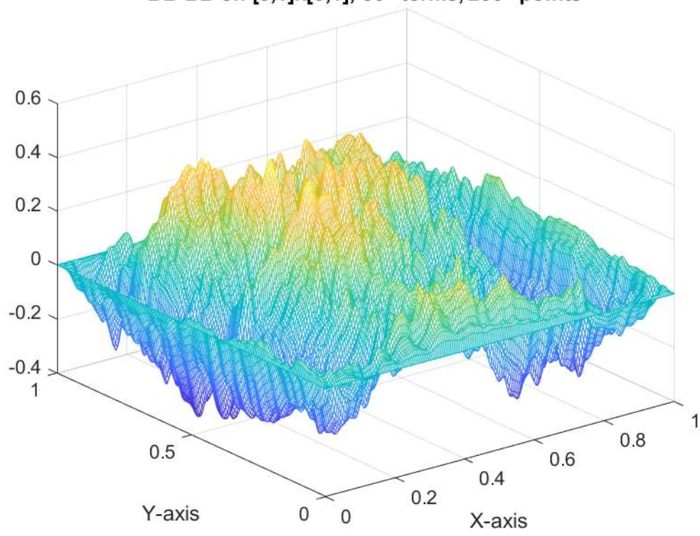
BB-BB on [0,1] \times [0,1] ; 80^2 terms, 200^2 points
