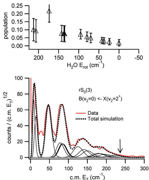
Figure 7. Fragment translational energy distribution (c.m.) obtained by monitoring \text{NH}_3(v_2 = 2^+, J = 3, K = 0) via the rS_0(3) line of the \bar{B} \leftarrow \bar{X} transition and simulation (see text for details). The arrow indicates the maximum available translational energy for D_0 = 1538 \text{ cm}^{-1} . The top panel shows the normalized relative populations of the water rotational states used to fit the data. The x -axis has been inverted such that the states line up vertically with the corresponding features in the c.m. translational energy distribution.
