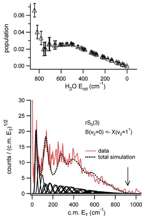
Figure 8. Fragment translational energy distribution (c.m.) obtained by monitoring \text{NH}_3(v_2 = 1^+, J = 3, K = 0) via the rS_0(3) line of the \bar{B} \leftarrow \bar{X} transition and simulation (see text for details). The arrow indicates the maximum available translational energy for D_0 = 1538 \text{ cm}^{-1} . The top panel shows the normalized relative populations of the water rotational states used to fit the data. The x -axis has been inverted such that the states line up vertically with the corresponding features in the c.m. translational energy distribution.
