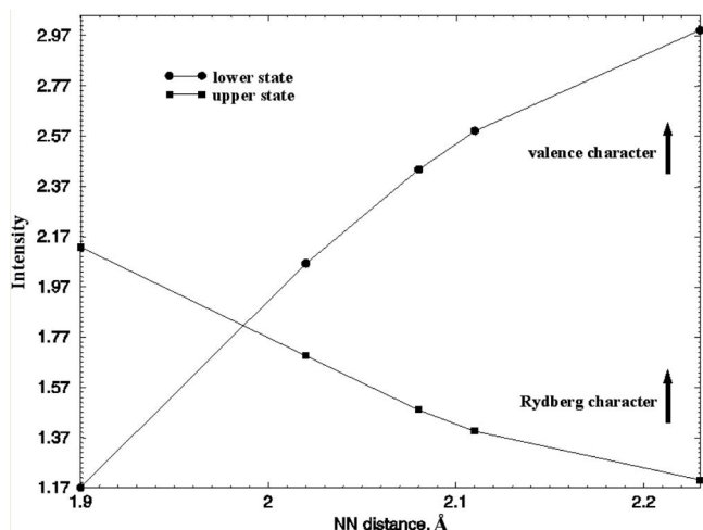
FIG. 8. The dependence of the absorption intensity \langle \bar{\mu}_{\text{elec}} \rangle^2 vs R(\text{N}-\text{N}) for the two B_2 transitions of mixed Rydberg ( 3p_y ) and valence ( \sigma_d \rightarrow \sigma_d^* ) character, from the EOM-EE-CCSD runs of Fig. 7.
