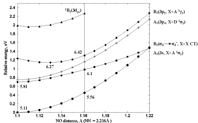
FIG. 10. EOM-EE-CCSD/6-311(2+)G(2df) results for selected dimer states, as a function of symmetric R(\text{N}-\text{O}) stretch. The R(\text{N}-\text{N}) and \angle \text{ONN} values were taken to be 2.236 Å and 99.6° (Ref. 42). The zero of energy corresponds to the “minimum” of the {}^1A_1(3s) state. Vertical and “adiabatic” [with R(\text{N}-\text{N}) and \angle \text{ONN} fixed] excitation energies are also shown. The characters of the {}^1B_2 states are inverted at smaller \text{N}-\text{N} distances due to an avoided crossing, similar to the crossing in Fig. 7.
