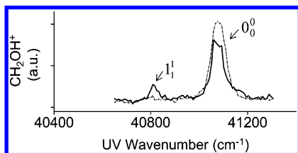
Figure 3. IR+UV double resonance spectrum of \text{CH}_2\text{OH}^+ via the 3p_z state with IR off (dot dashed line) and IR tuned to the OH stretch at 3674.3 \text{ cm}^{-1} (solid line).
