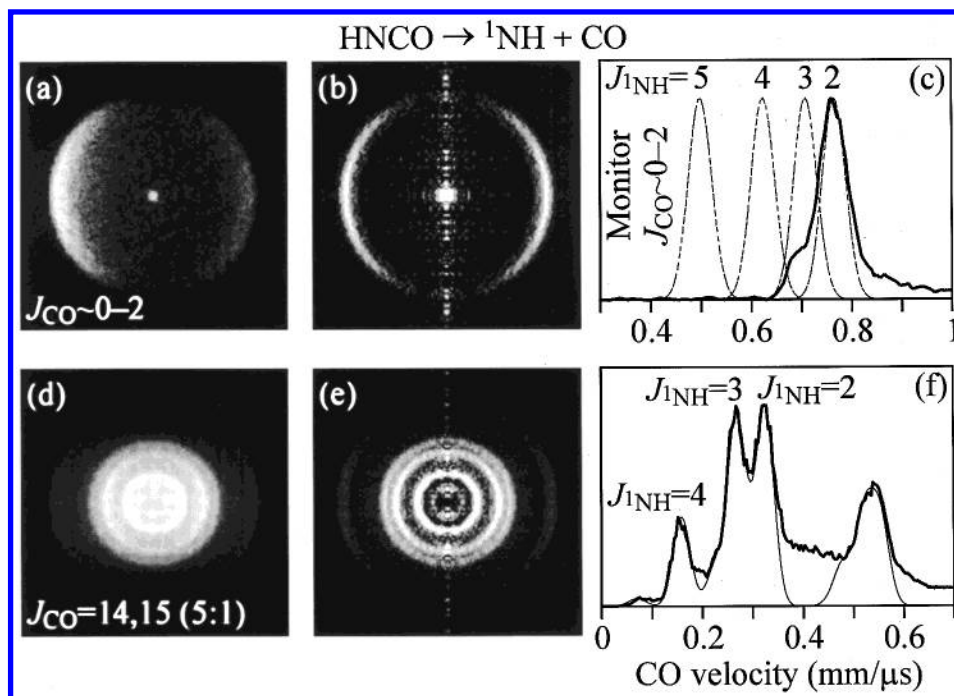
FIGURE 2. CO images obtained at \sim 230.1 nm in a one-color experiment monitoring (a) J_{\text{CO}} = 0-2 and (d) J_{\text{CO}} = 14, 15 . Panels (b) and (e) represent 2D cuts through the 3D velocity distributions of images (a) and (d), respectively. In panels (c) and (f) the corresponding velocity distributions derived from the reconstructed 3D images are shown in thick lines. The thin dashed lines in (c) show positions of {}^1\text{NH} levels. The thin solid lines in (f) show fits to the velocity distributions. The feature at \sim 0.5 mm/ \mu\text{s} in (f) is from dissociation of a hot band.
