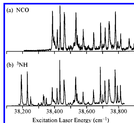
FIGURE 3. Photofragment yield spectra of HNCO obtained in the region near the threshold of channel 2 obtained by monitoring (a) NCO and (b) {}^3\text{NH} , while scanning the photolysis laser.
