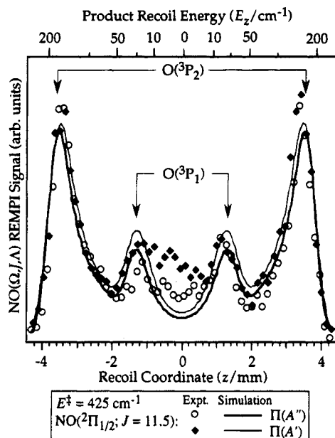
Figure 8. Spatial profiles of \text{NO}(^2\Pi_{1/2}; J=11.5) obtained at E^{\ddagger} = 425 \text{ cm}^{-1} and their least-squares fits. The Q_{11} + P_{21}(11.5) line was used to obtain the spatial distribution of NO in the \Pi(A'') \Lambda -doublet state, while the R_{11} + Q_{21}(11.5) transition was used to detect NO in the \Pi(A') state. The arrows indicate the peaks correlated with the ^3P_2 and ^3P_1 spin-orbit states of the O atom. See Figure 4 for other details.
