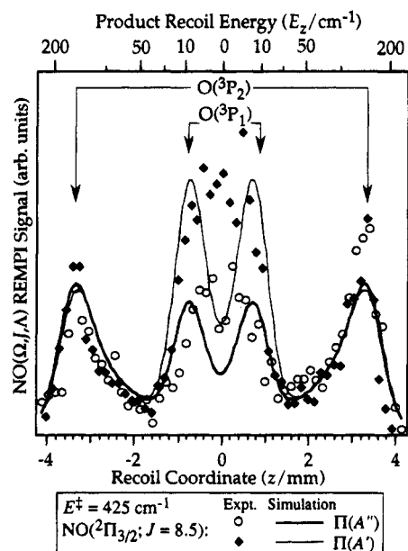
Figure 9. Spatial profiles of \text{NO}(^2\Pi_{3/2}; J=8.5) obtained at E^{\ddagger} = 425 \text{ cm}^{-1} and their least-squares fits. The Q_{22} + R_{12}(8.5) line was used to obtain the spatial distribution of NO in the \Pi(A'') \Lambda -doublet state, while the R_{22}(8.5) transition was used to detect NO in the \Pi(A') state. The arrows indicate the peaks correlated with the ^3P_2 and ^3P_1 spin-orbit states of the O atom. See Figure 4 for other details.
