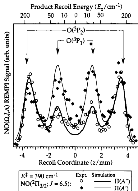
Figure 5. Spatial profiles of NO( ^2\Pi_{3/2}; J = 6.5 ) obtained at E^\ddagger = 390 \text{ cm}^{-1} and their least-squares fits. The Q_{22} + R_{12}(6.5) line was used to obtain the spatial distribution of NO in the \Pi(A'') \Lambda -doublet state, while the R_{22}(6.5) transition of NO was used to detect NO in the \Pi(A') state. The arrows indicate the peaks correlated with the ^3P_2 and ^3P_1 spin-orbit states of the O atom. See Figure 4 for other details.
