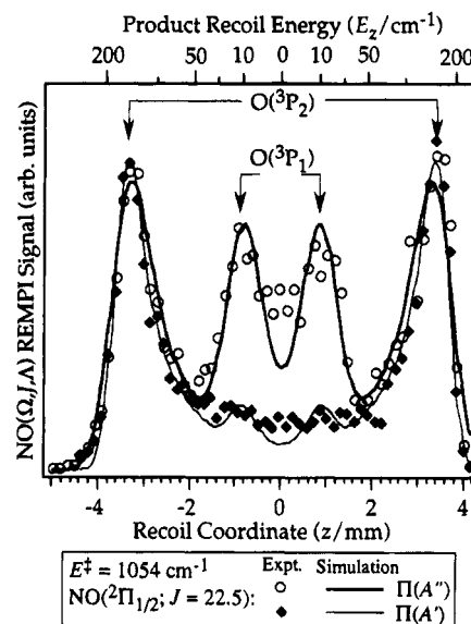
Figure 10. Spatial profiles of \text{NO}(^2\Pi_{1/2}; J=22.5) obtained in \text{NO}_2 photodissociation at E^{\ddagger} = 1054 \text{ cm}^{-1} and their least-squares fits. The Q_{11} + P_{21}(22.5) line was used to obtain the spatial distribution of NO in the \Pi(A'') \Lambda -doublet state, while the R_{11} + Q_{21}(22.5) transition was used to detect NO in the \Pi(A') state. The arrows indicate the peaks correlated with the ^3P_2 and ^3P_1 spin-orbit states of the O atom. See Figure 4 for other details.
