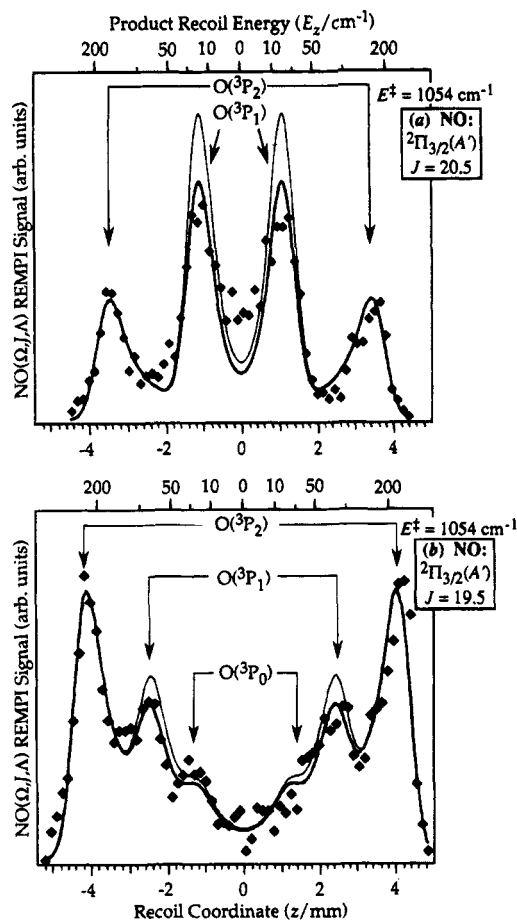
Figure 11. Spatial profiles of (a) NO( ^2\Pi_{3/2}; J=20.5; \Pi(A') ) and (b) NO( ^2\Pi_{3/2}; J=19.5; \Pi(A') ) obtained in NO 2 photodissociation at E^* = 1054 \text{ cm}^{-1} (symbols). The spatial distributions were obtained by monitoring the P_{22} + Q_{12}(20.5) and P_{22} + Q_{12}(19.5) transitions, respectively. The least-squares fits are shown by the thick lines. Shown by the thin lines are the simulations obtained by increasing the O( ^3P_1 ):O( ^3P_2 ) ratio by 30% compared to the values obtained from the least-squares fits. The arrows indicate the peaks correlated with the ^3P_2 , ^3P_1 and ^3P_0 spin-orbit states of the O atom. See Figure 4 for other details.
