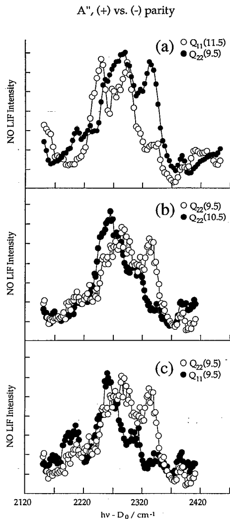
FIG. 11. PHOFRY spectra of NO 2 which compare the spectrum obtained by monitoring the Q 22 (9.5) transition of the (0,0) band of the NO \gamma system with those obtained by monitoring (a) the Q 11 (11.5); (b) the Q 22 (10.5), and (c) the Q 11 (9.5) transitions of the same band [(a) CI_{rms}=0.075 ; (b) 0.062; and (c) 0.057]. These transitions access NO rovibrational levels of similar total angular momentum and the same electronic parity, but different total parity.
