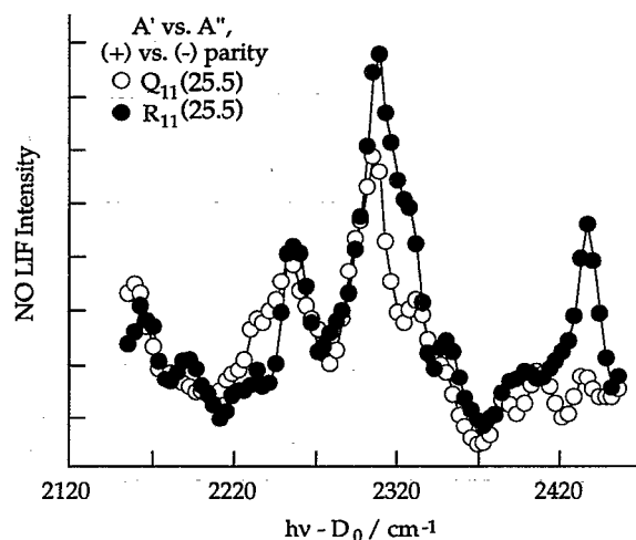
FIG. 17. PHOFRY spectra of NO 2 obtained by monitoring the Q_{11} (25.5) and R_{11} (25.5) transitions of the (0,0) band of the NO \gamma system ( CI_{\text{rms}}=0.021 ). These transitions access NO rovibrational levels of different electronic and total parity.
