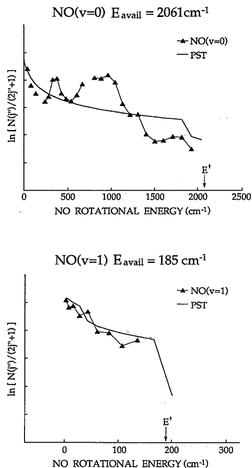
FIG. 5. Rotational state distributions of the NO( ^2\Pi_{1/2}, v=0 ) and NO( ^2\Pi_{1/2}, v=1 ) fragments following NO 2 photolysis at E^\ddagger=2061 cm -1 , summed over \Lambda -doublet levels.
