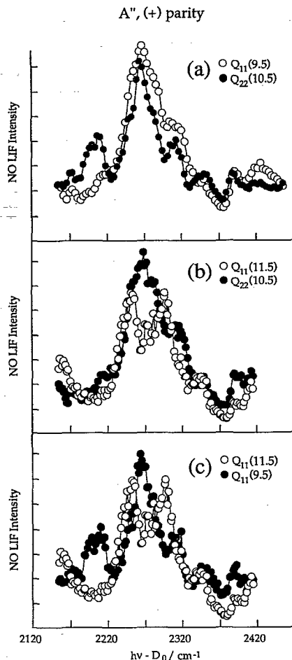
FIG. 13. PHOFRY spectra of NO 2 obtained by monitoring (a) the Q 11 (9.5) and Q 22 (10.5) transitions; (b) the Q 11 (11.5) and Q 22 (10.5) transitions; and (c) the Q 11 (11.5) and Q 11 (9.5) transitions of the (0,0) band of the NO \gamma system [(a) CI_{\text{rms}}=0.032 ; (b) 0.026; and (c) 0.074]. These transitions access NO rovibrational levels of the same electronic and total parity.
