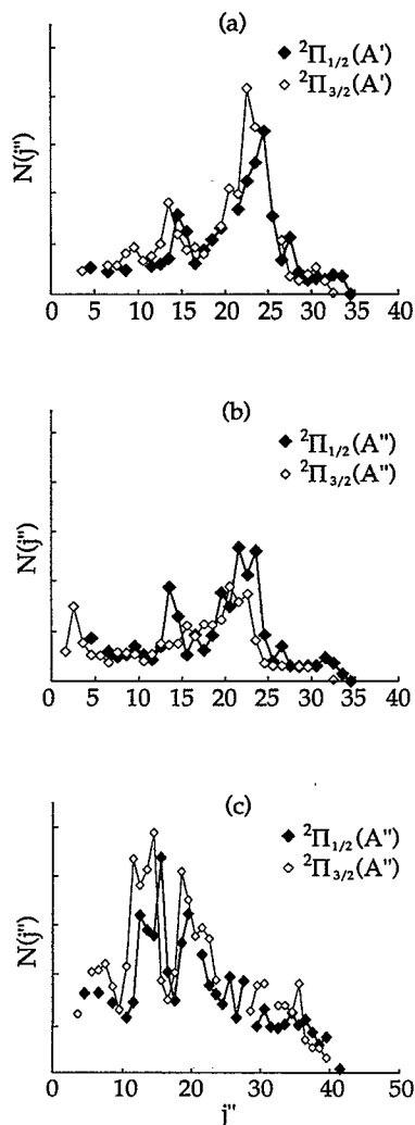
FIG. 4. Rotational state distributions of the NO( ^2\Pi_{1/2}, v=0 ) and NO( ^2\Pi_{3/2}, v=0 ) fragments following NO 2 photolysis at excess energies ( E^\ddagger ) of (a) and (b) 2061; and (c) 3038 cm -1 . In this figure, the rotational distributions of the individual \Lambda -doublet levels of the two spin-orbit states are shown. Note the consistent shift of the ^2\Pi_{3/2} distribution with respect to that in the ^2\Pi_{1/2} state.
