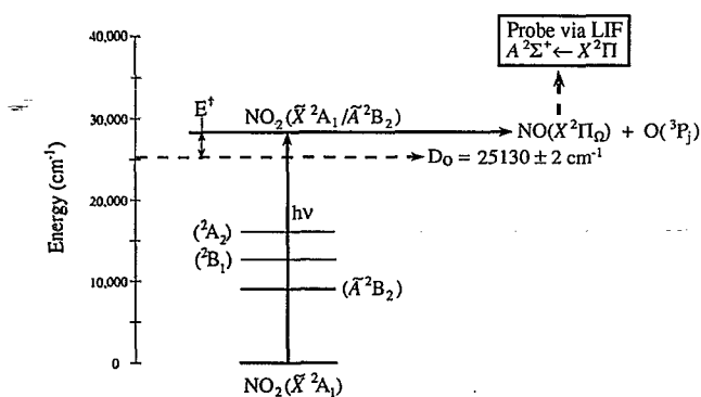
FIG. 1. An energy level diagram of NO 2 . Single photon excitation from the ground ^2A_1 state prepares eigenstates of predominantly ( ^2B_2/2A_1 ) character, which are optically accessed via the allowed ( ^2B_2 \leftarrow ^2A_1 ) transition.
