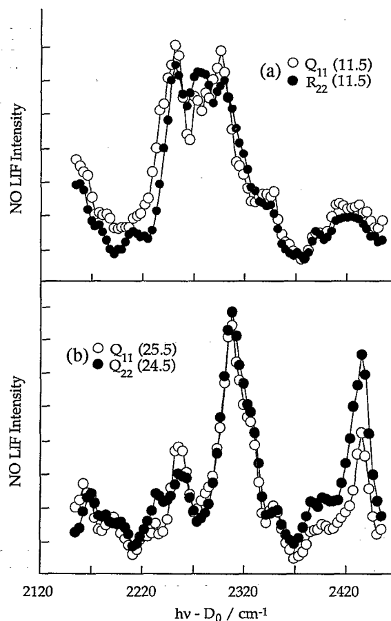
FIG. 7. PHOFRY spectra of NO 2 at E^\ddagger = 2150 – 2450 cm -1 obtained by monitoring (a) the Q_{11}(11.5) and R_{22}(11.5) transitions; and (b) the Q_{11}(25.5) and Q_{22}(24.5) transitions of the NO (0,0) band. These spectra reveal a correlation based on total angular momentum.
