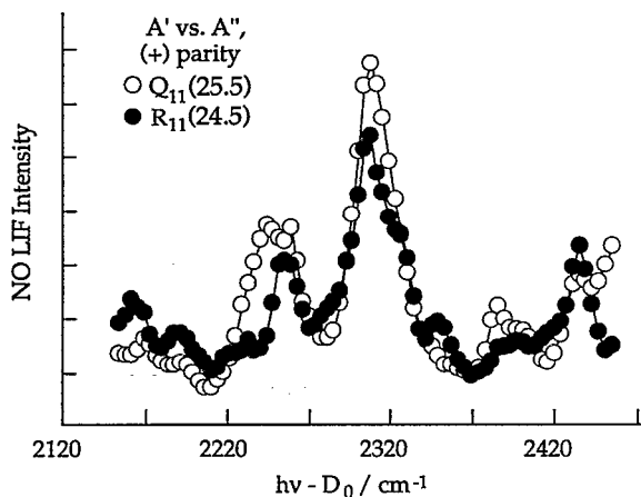
FIG. 15. PHOFRY spectra of NO 2 obtained by monitoring the Q_{11} (25.5) and R_{11} (24.5) transitions of the (0,0) band of the NO \gamma system ( CI_{\text{rms}}=0.033 ). These transitions access NO rovibrational levels of the same total parity, but different electronic parity.
