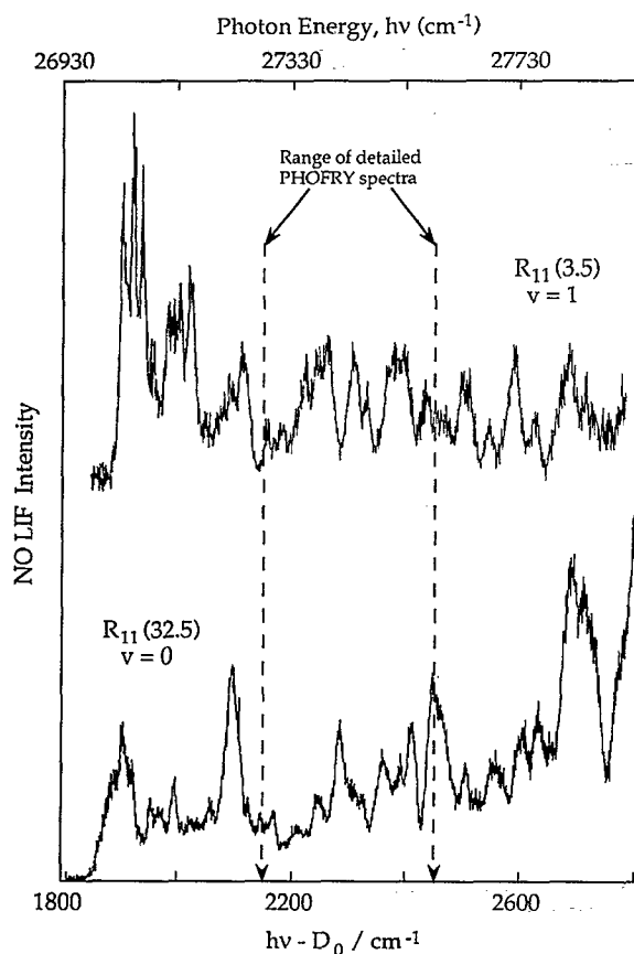
FIG. 6. Photofragment yield (PHOFRY) spectra of NO 2 at E^\ddagger = 1800 – 2800 cm -1 obtained by monitoring the R_{11}(3.5) and R_{11}(32.5) transitions, respectively, of the (1,1) and (0,0) bands of the NO \gamma system. The energy appearance thresholds for these two levels are similar. Note the degree of structure which persists to E^\ddagger = 2800 cm -1 .
