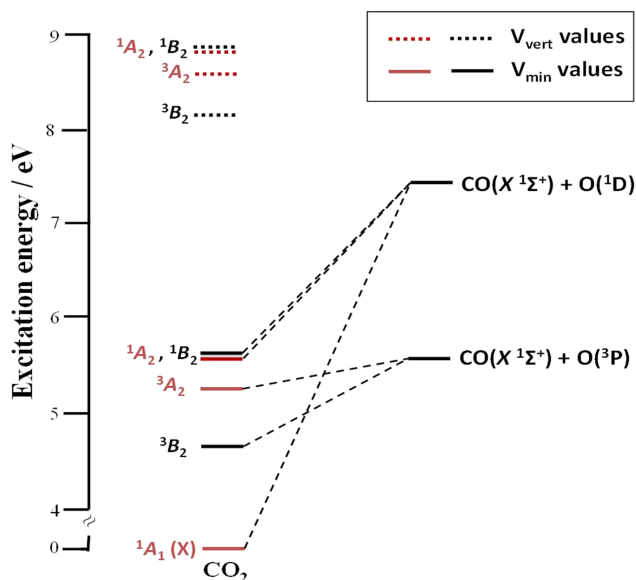
FIG. 7. Energy diagram showing adiabatic ( V_{\min} , solid line) and vertical ( V_{\text{vert}} , dashed line) energies of the excited electronic states of \text{CO}_2 listed in Table I. A and B states are shown in red and black, respectively.
