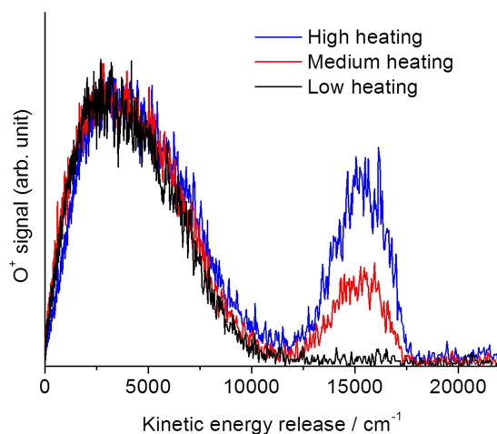
FIG. 5. c.m. KER distributions obtained by monitoring O( 3 P 2 ) products at 225.654 nm with low (black), medium (red), and high (blue) CO 2 heating. The intensities of the KER distributions obtained with different heating levels are normalized with respect to the broad feature centered at \sim 3000\text{ cm}^{-1} .
