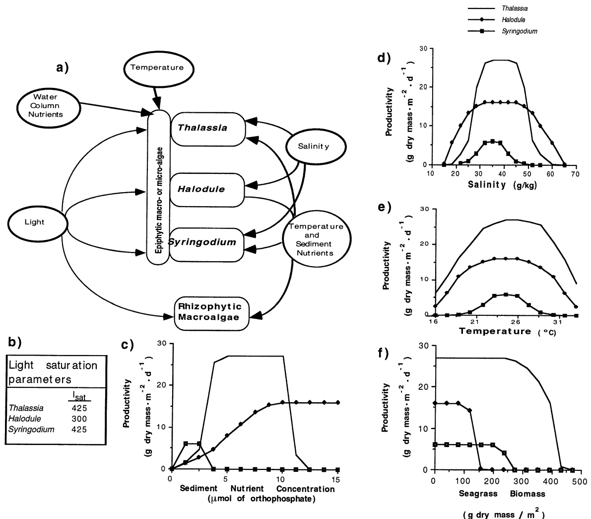
FIG. 1. (a) Conceptual model of seagrass ecosystem, and graphical representation of model relationships between productivity of seagrass and (b) light, (c) sediment nutrients (pore water + water extractable), (d) water salinity, (e) temperature, and (f) seagrass biomass.
